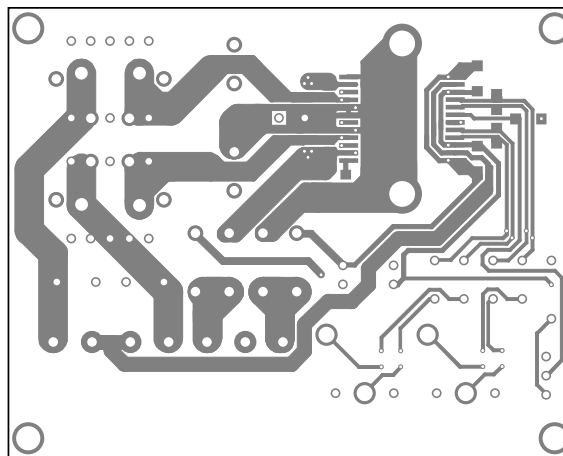
Top copper
